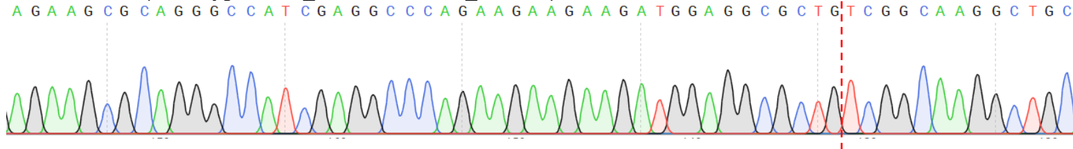
Figure S4: CAMSAP1 sequencing chromatograms from Family 1
