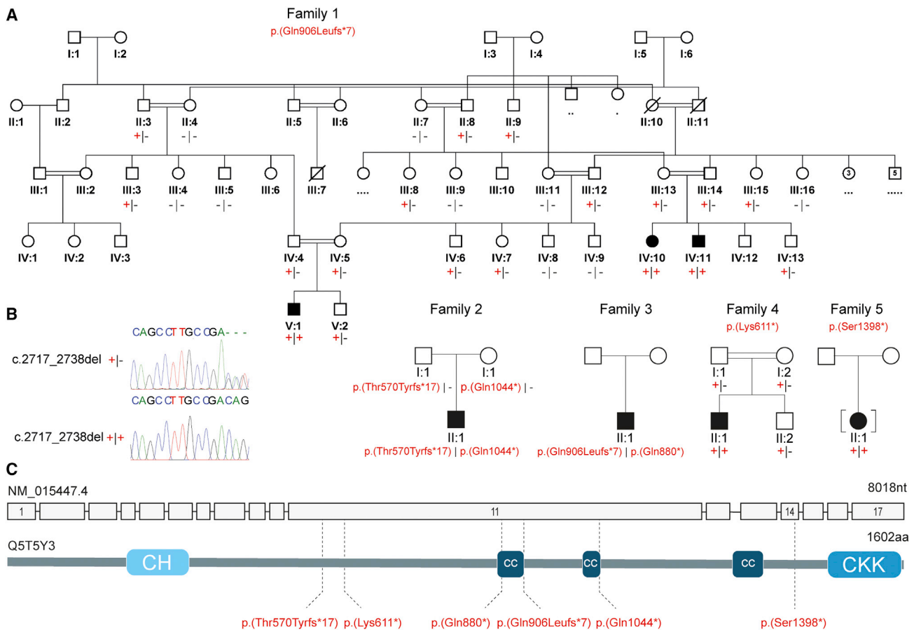
Figure 1. Family pedigrees and bi-allelic CAMSAP1 variants associated with a syndromic neuronal migration disorder
