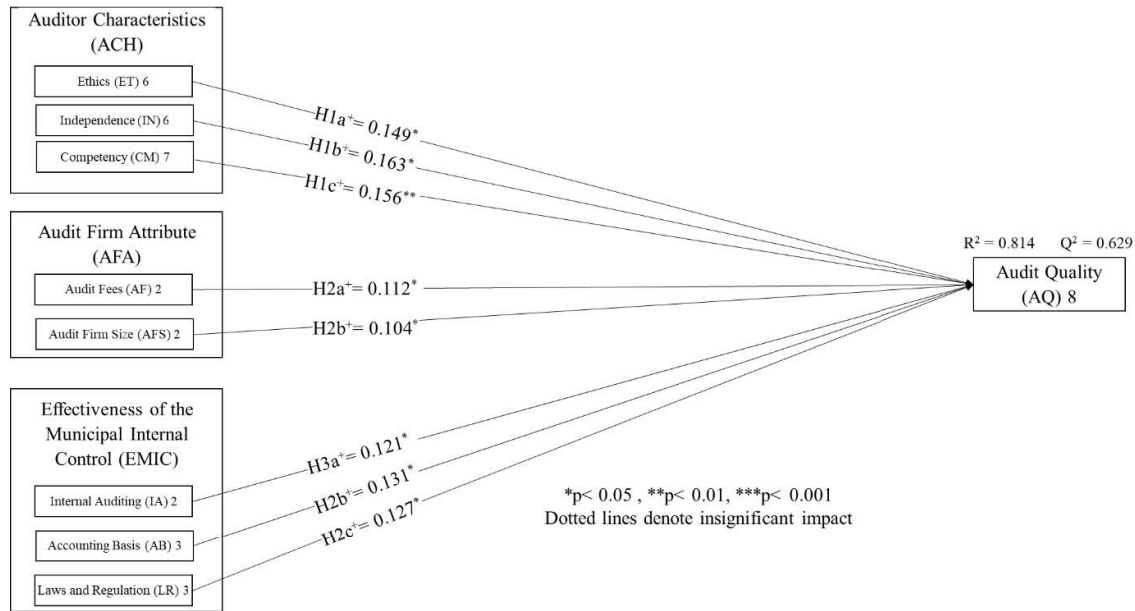
Figure 2: Direct Effect Hypotheses - Structural Model
