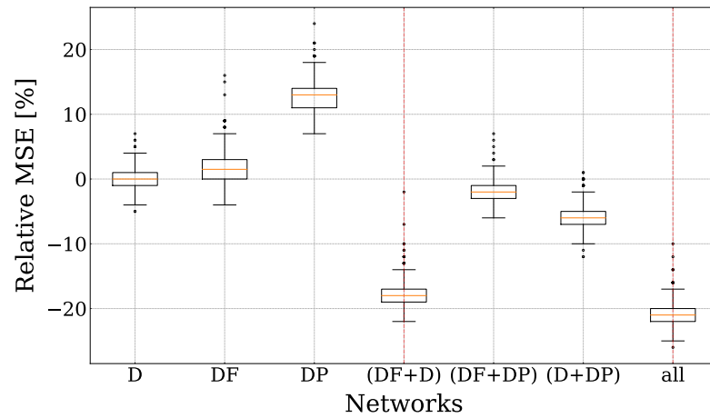
Figure 7. Boxplots represent the training MSE results of the algorithms using UX, N = 20, 24, 30 samples with complexity (3, 2) . The x-axis represents the algorithm inputs we applied, and the y-axis denotes the relative MSE calculated, with D -input algorithms as a reference case.
